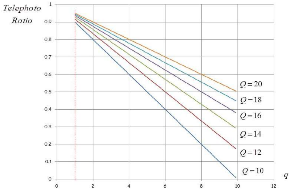
Fig 5. Telephoto ratio as function of q , for several values of Q .
